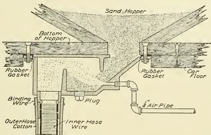
Fig. 123. Section of Pneumatic Sander
